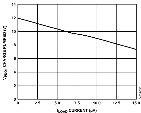
Figure 11. V PDO1 (FET Drive Mode) vs. I LOAD
