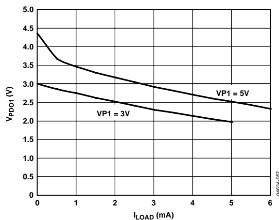
Figure 12. V PDO1 (Strong Pull-Up to VPn) vs. I LOAD
