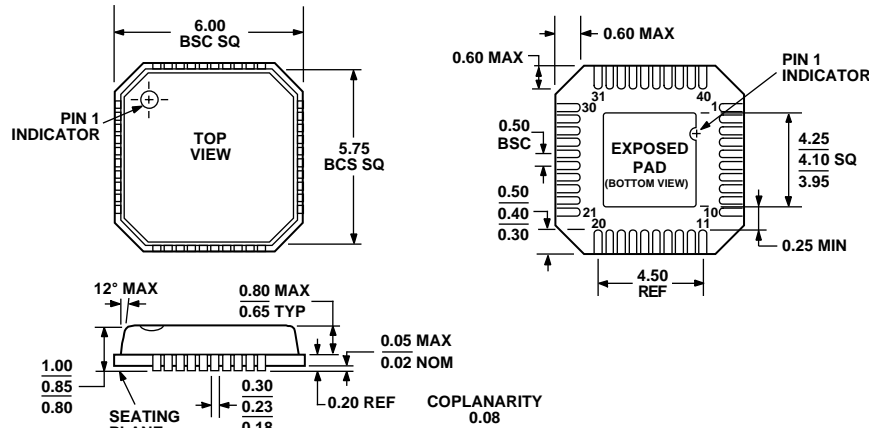
Figure 38. 40-Lead Lead Frame Chip Scale Package [LFCSP_VQ] 6 mm × 6 mm Body, Very Thin Quad (CP-40)
