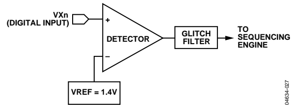
Figure 18. VXn Digital Input Function
