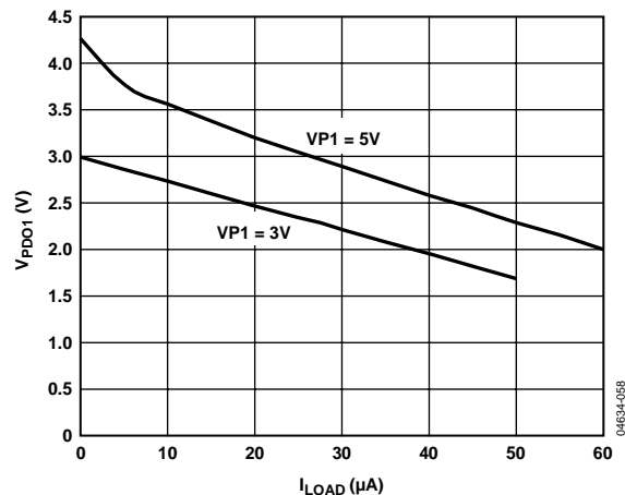
Figure 13. V PDO1 (Weak Pull-Up to VPn) vs. I LOAD
